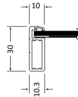
Frame short side cross section
